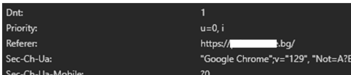
Figure 4. Without a restrictive Referrer-Policy, the URL of the origin of the request is being shared with the target
